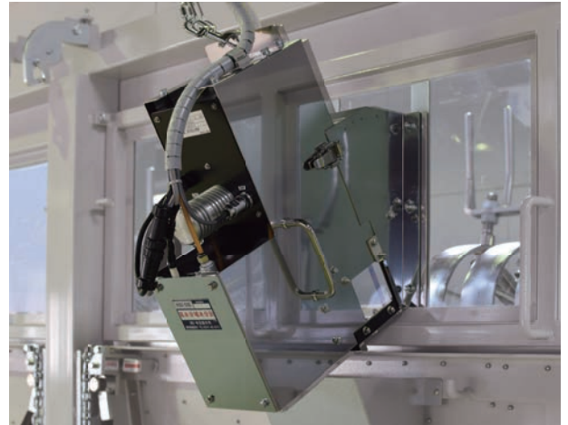
Near infrared moisture measuring sampling unit (For high moisture range) ASU-SSE
